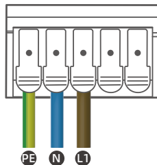
TN 1-phasig (230V)
