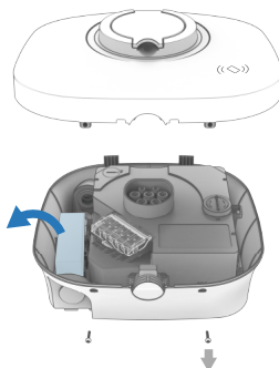
TX10 Torx screw M3x16mm x 2
